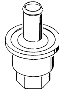
FIG. 8 18mm I.D. Hose M24X2.0 Thread
