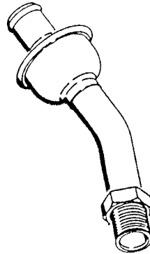
FIG. 3 3/4" I.D. Hose 3/4" - 14 Dryseal PTF Thread
