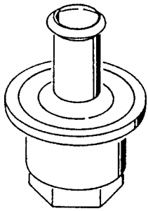
FIG. 1 1/2" to 3/4" I.D. Hose Size 3/4" - 14 NPSF Thread
