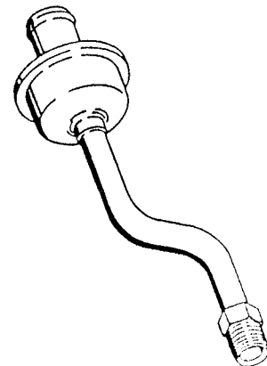
FIG. 12 3/4" I.D. Hose 1/2" - 18 NPSF Thread
